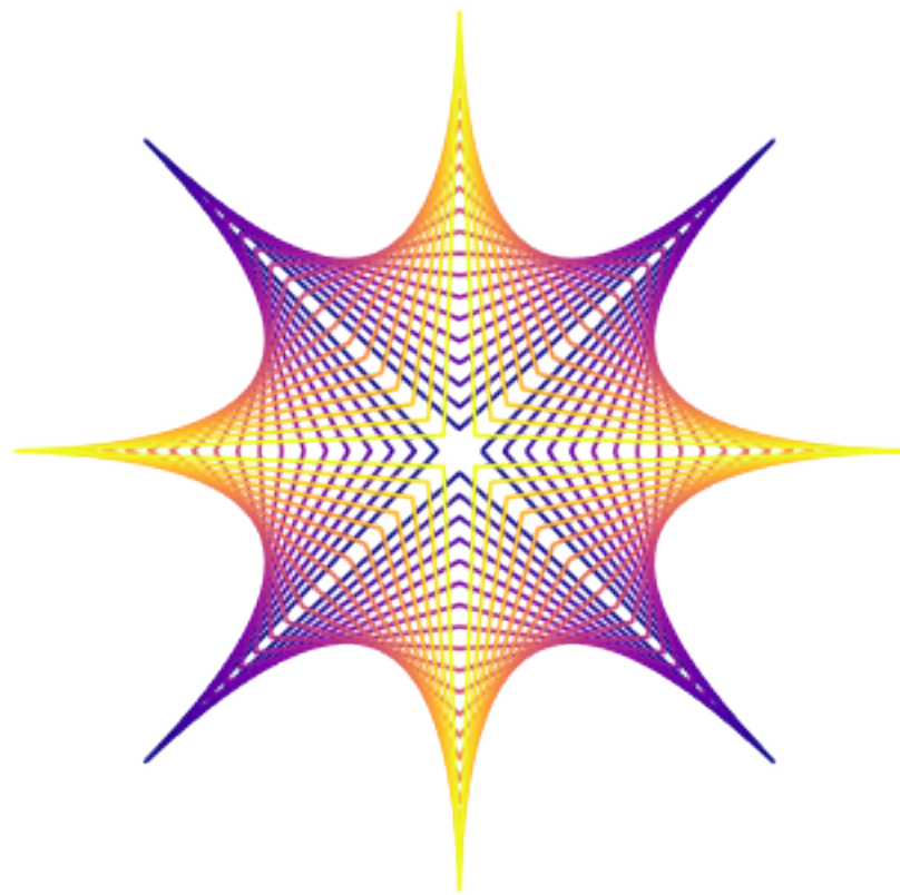
plasma
