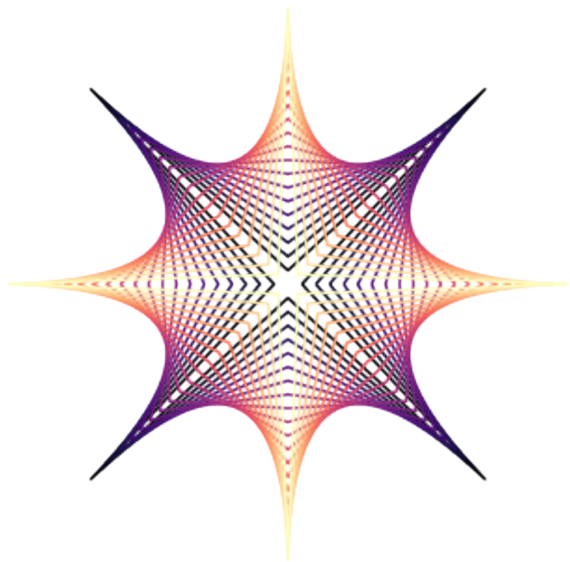
magma
